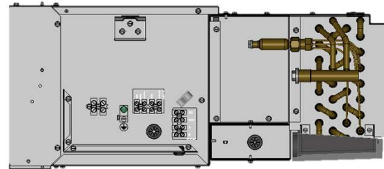
Main power connections
