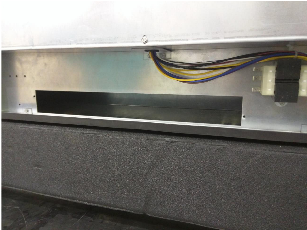
Indoor unit- heater kit installation site
