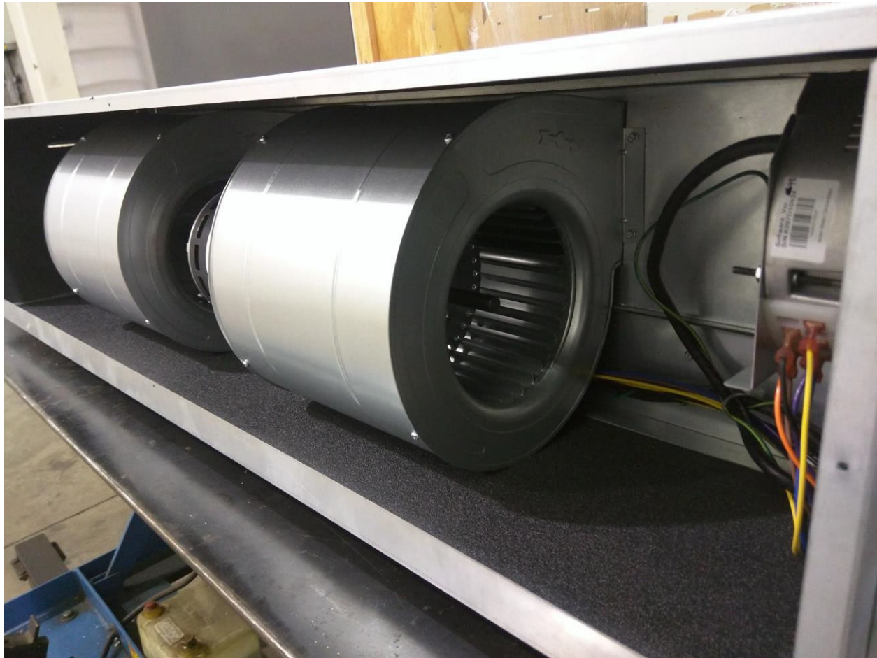
Indoor unit - motor compartment
