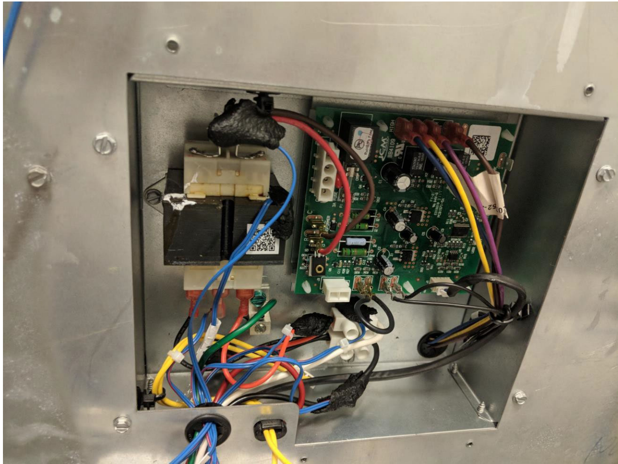
Indoor unit - field wiring compartment
