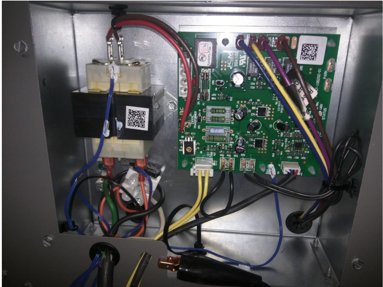
Control compartment
