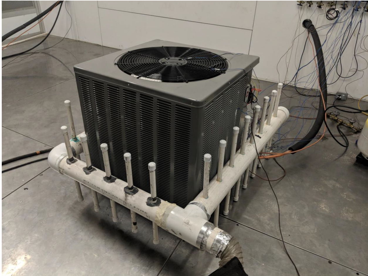
Outdoor unit - exterior back
