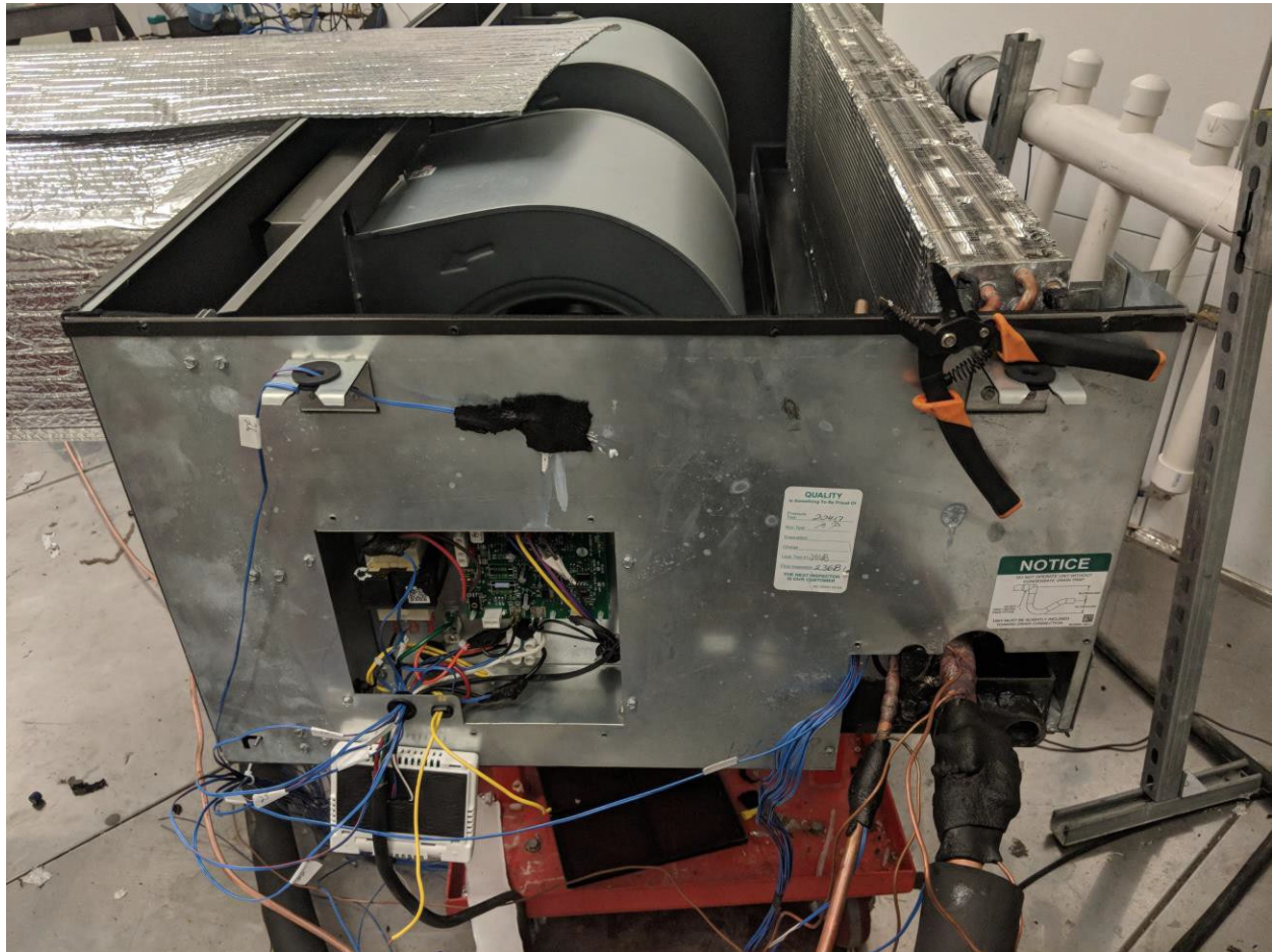
Indoor unit - exterior on wiring compartment side
