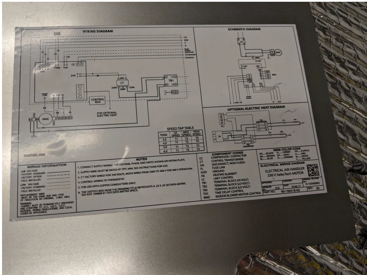
Indoor unit - wiring diagram
