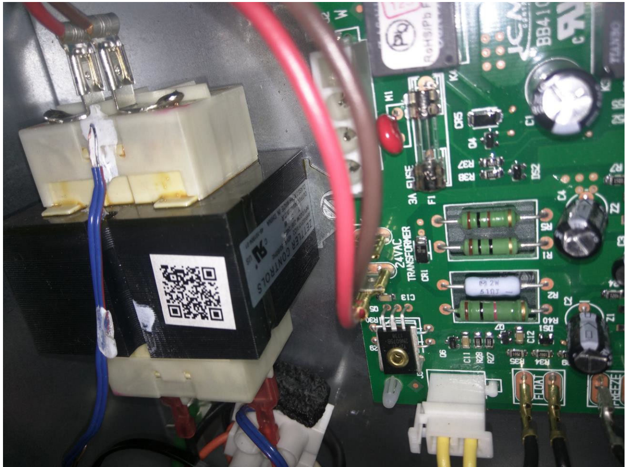
Transformer
